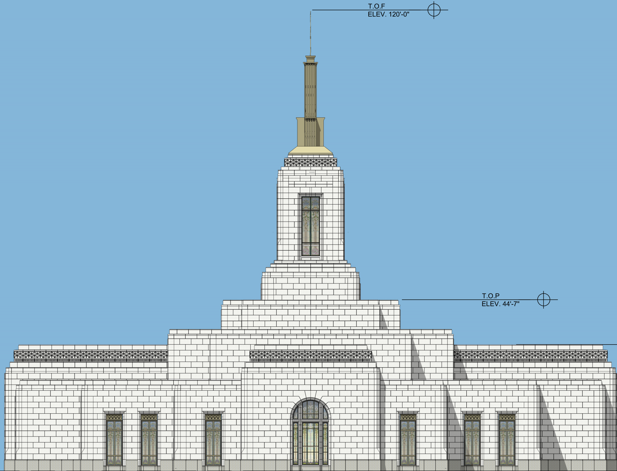
BACK (NORTH) ELEVATION - MCKINNEY TEMPLE
